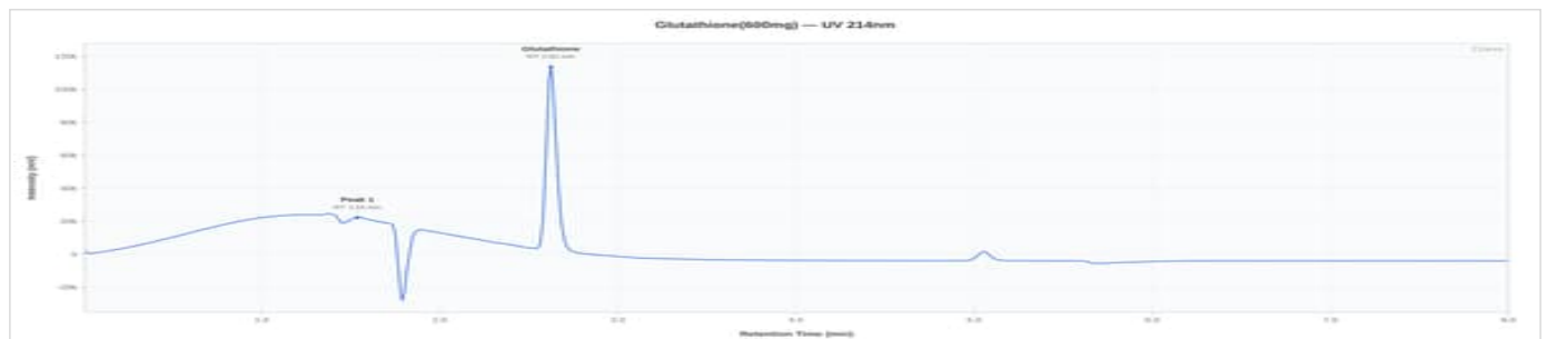
Glutathione 600mg - GLUTA0001: UV Chromatogram
