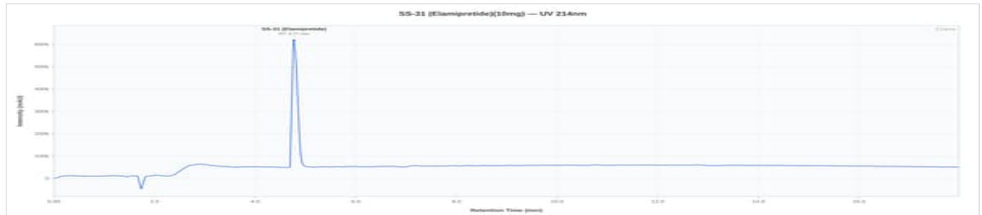
SS-31 10mg - SS310001: UV Chromatogram
