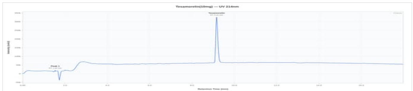
Tesamorelin 10mg - TESA0001: UV Chromatogram
